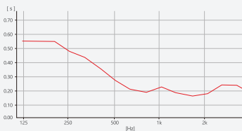
Reverberation time test
