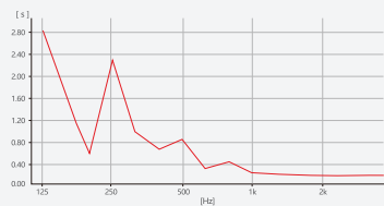
Reverberation time test
