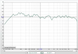
Frequency response
