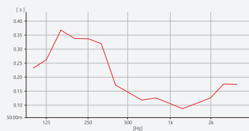
Reverberation time test
