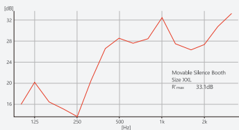
Sound insulation test
