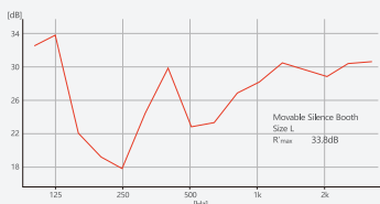
Sound insulation test
