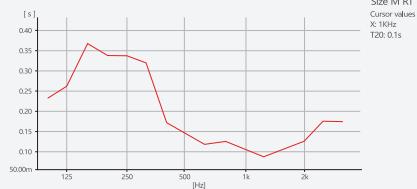
Reverberation time test
