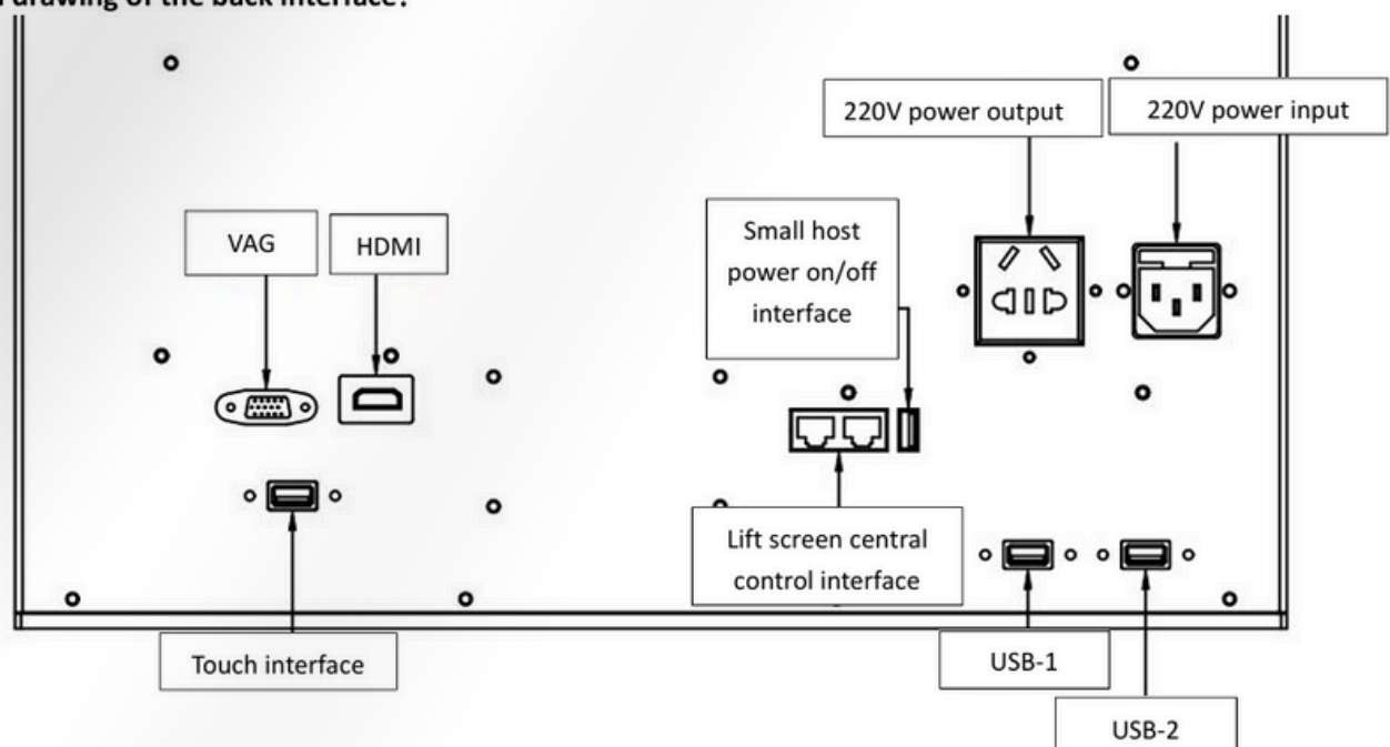
Detail drawing of the back interface:
